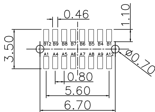
RECOMMENDED P.C.B LAYOUT TOP VIEW TOLERANCE UNSPECIFIED \pm 0.05\text{mm}
