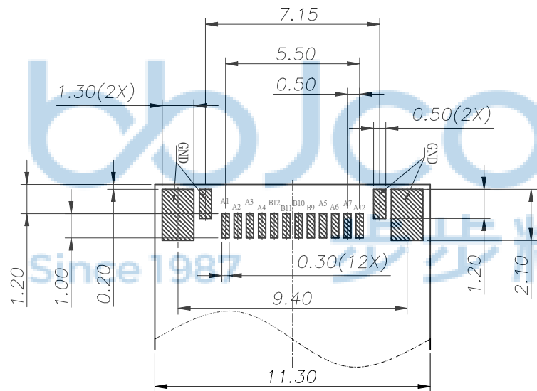
RECOMMENDED PCB LAYOUT(TOP VIEW)
