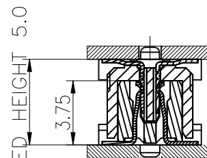
MATED HEIGHT
