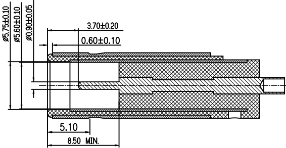
MATING PLUG DP790090-0145-60000H
