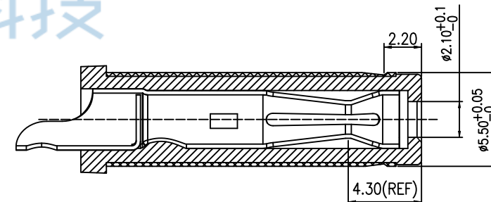
MATING PLUG
