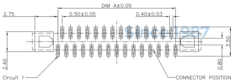
RECOMMENDED P.C.B PATTERN LAYOUT
