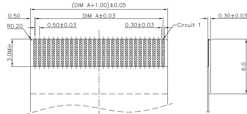
RECOMMENDED FPC/FFC DIMENSIONS
