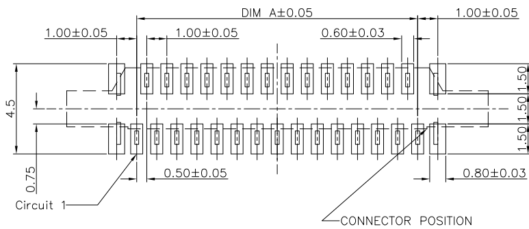
RECOMMENDED P.C.B. PATTERN LAYOUT
