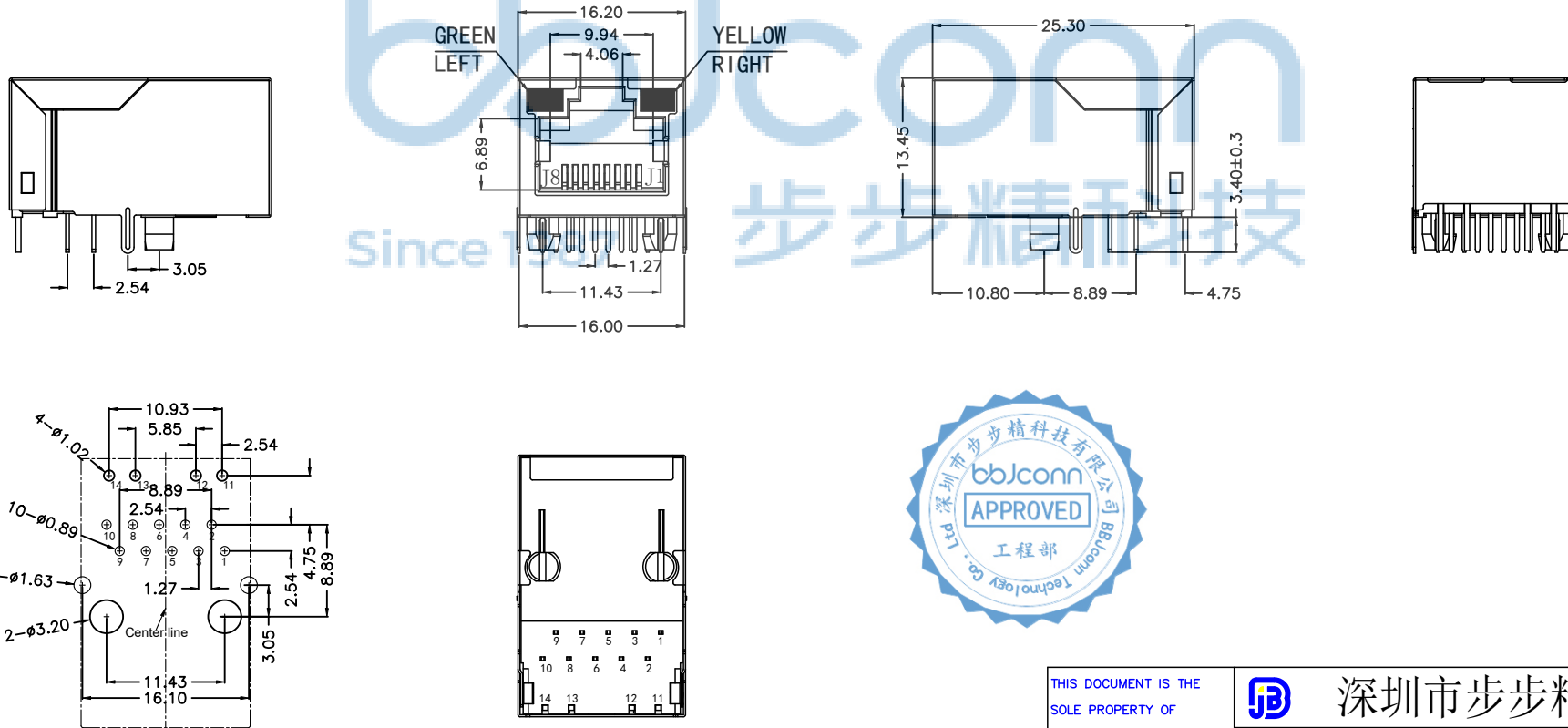
RECOMMENDED PCB LAYOUT VIEWED FROM COMPONENT SIDE
