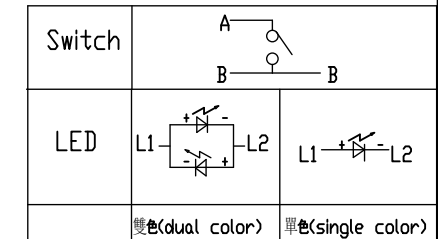
ELECTRICAL SCHEMATIC
