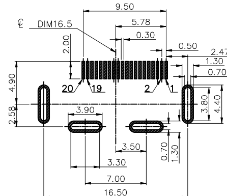
RECOMMEND PCB LAYOUT TOP VIEW
