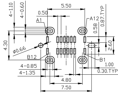
PCB LAYOUT ±0.05
