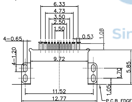
RECOMMENDED PCB LAYOUT(TOP VIEW) DEFAULT TOLERANCE:±0.05
