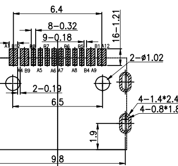
RECOMMENDED PCB LAYOUT Tolerance: ±0.05mm
