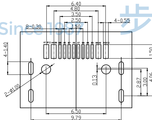
RECOMMENDED P.C.B. LAYOUT TOLERANCE UNSPECIFIED \pm 0.05\text{mm}
