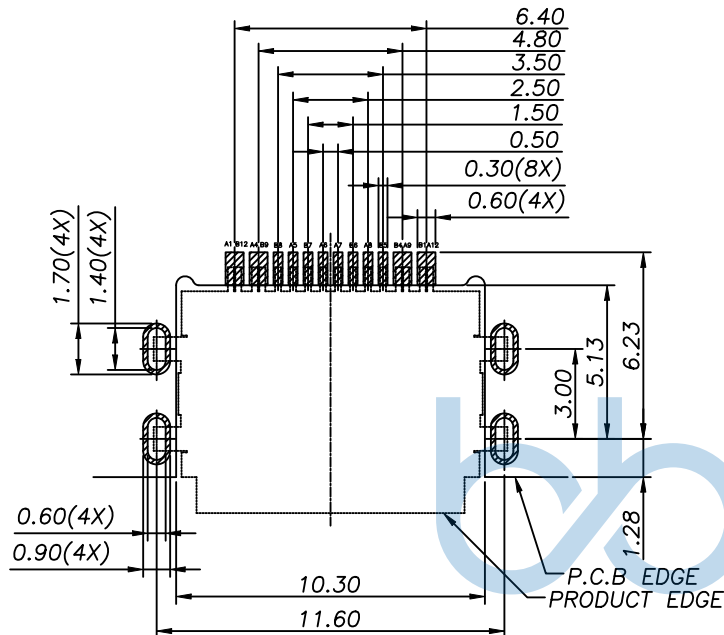
RECOMMENDED P.C.B. LAYOUT TOLERANCE UNSPECIFIED \pm 0.05\text{mm}
