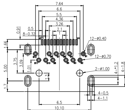
RECOMMENDED PCB LAYOUT Tolerance: \pm 0.05\text{mm}
