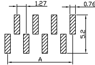
RECOMMEND P. C. B LAYOUT PCB TOLERANCE: ±0.05 (TOP VIEW)
