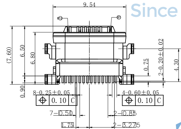
Mated Condition(REF.)
