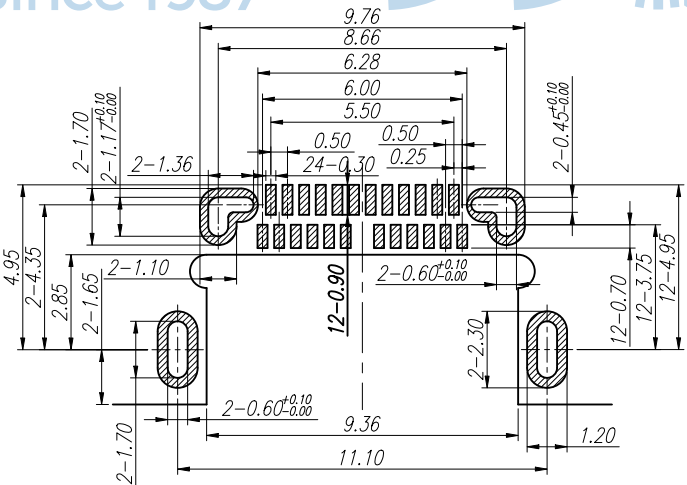
P.C.B LAYOUT VIEW TOLERANCE ±0.05
