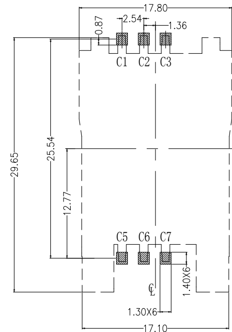
RECOMMENDED PCB LAYOUT TOLERANCE:±0.05
