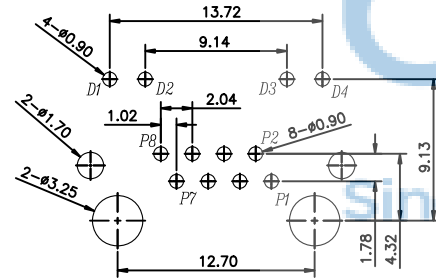
RECOMMENDED P.C.B LAYOUT TOP VIEW (COMPONENT SIDE)
