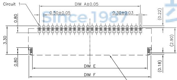
RECOMMENDED P.C.B PATTERN LAYOUT - CONNECTOR POSITION
