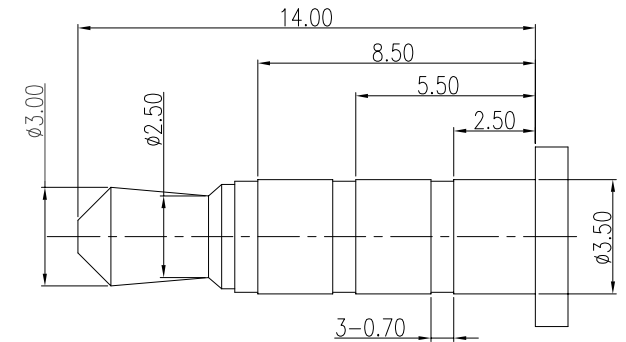
(ø3.50mm 4 POLE PLUG DETAIL DRAWING)
