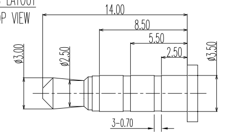
( \phi 3.50 mm 4 POLE PLUG DETAIL DRAWING)
