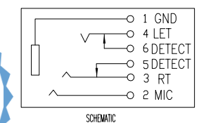
(ø3.50mm 4 POLE PLUG DETAIL DRAWING)
