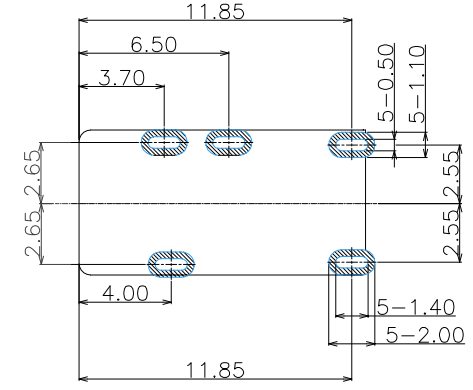
RECOMMEND FPC LAYOUT TOLERANCE : ±0.05
