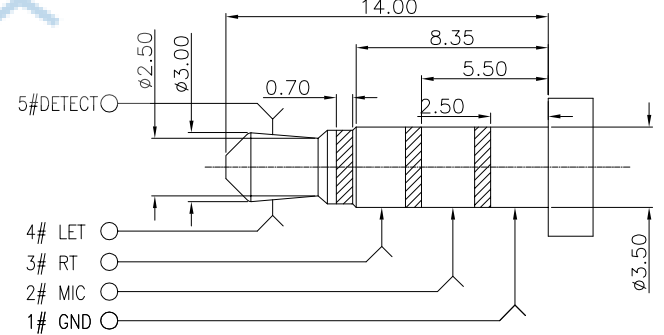
( \phi 3.50 mm 4 POLE PLUG DETAIL DRAWING)
