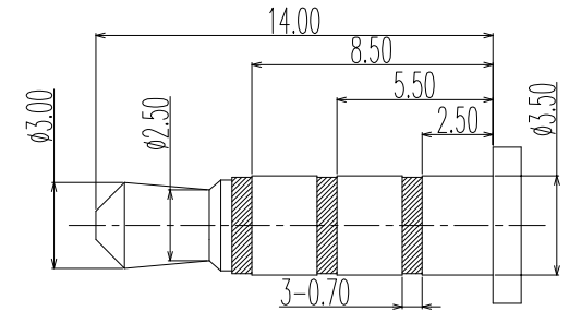
(∅3.50mm 4 POLE PLUG DETAIL DRAWING)
