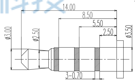
(φ3.50mm 4 POLE PLUG DETAIL DRAWING)
