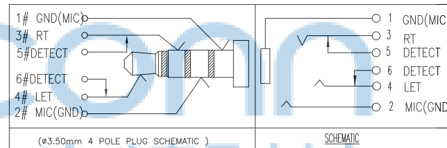
(φ3.50mm 4 POLE PLUG SCHEMATIC )
