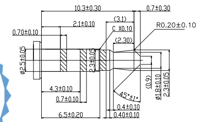
(ø2.50mm 4 POLE PLUG DETAIL DRAWING)
