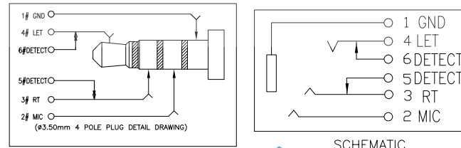
SCHEMATIC
