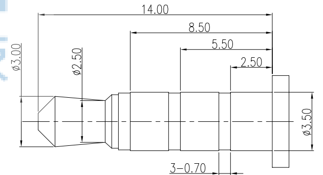
(ø3.50mm 4 POLE PLUG DETAIL DRAWING)
