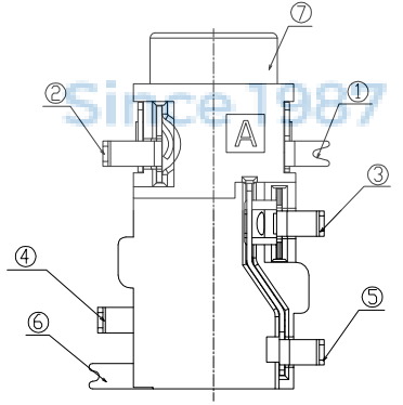
(ø3.50mm 4 POLE PLUG DETAIL DRAWING)
