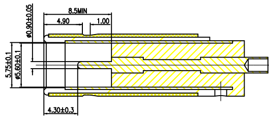
MATING PLUG
