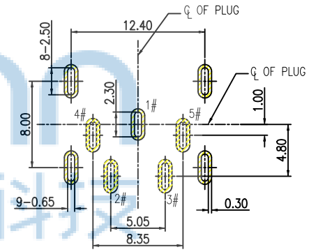
RECOMMENDED PCB LAYOUT TOP VIEW TOLERANCE: \pm 0.05
