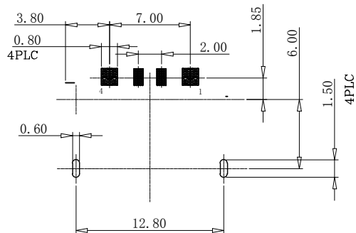
RECOMMENDED PCB LAYOUT THICKNESS=1.0mm (TOLERANCES ±0.05)
