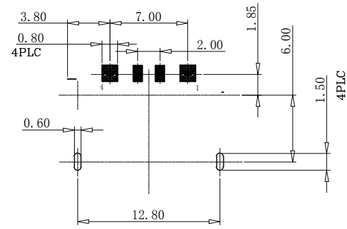
RECOMMENDED PCB LAYOUT THICKNESS=1.0mm (TOLERANCES ±0.05)
