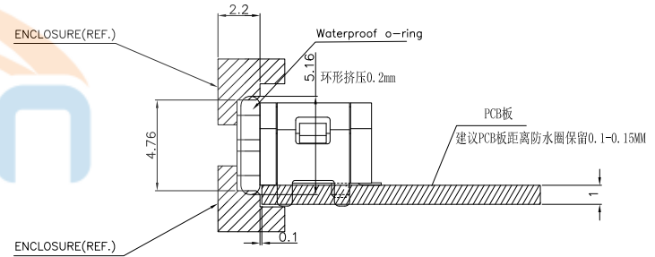
RECOMMENDED SCHEMATIC DRAWING OF CONNECTOR MATCH CHASSIS
