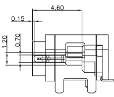
RECOMMENDED SCHEMATIC DRAWING OF CONNECTOR MATCH CHASSIS
