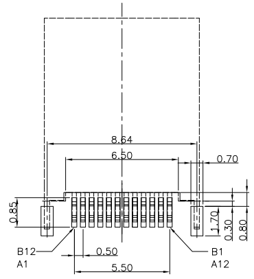
RECOMMENDED P.C.B. LAYOUT (T:1.00mm) TOLERANCE UNSPECIFIED ±0.05mm
